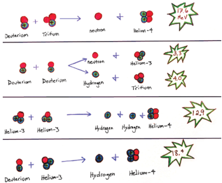
FIGURE 1 Fusion Reactions
