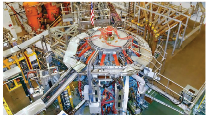
Fusion-Driver Program: National Spherical Torus Experiment (NSTX) facility.
