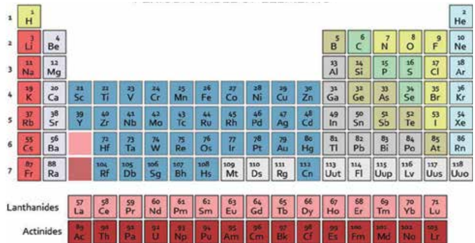
FIGURE 1 'Original' Periodic Table of Elements
